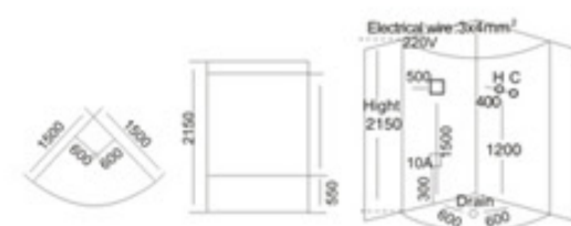
KB-884 1500x1500x2150mm
