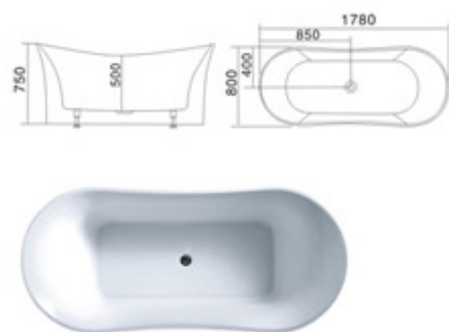
KB-512 1780x800x750mm
