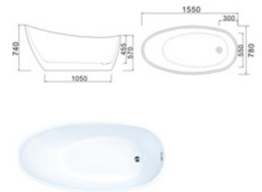
KB-534 1550x780x740mm
