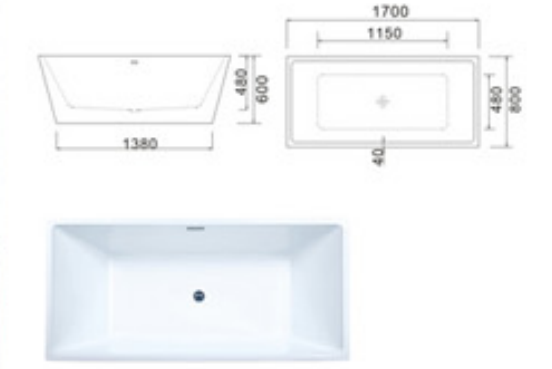
KB-522 1700x800x600mm
