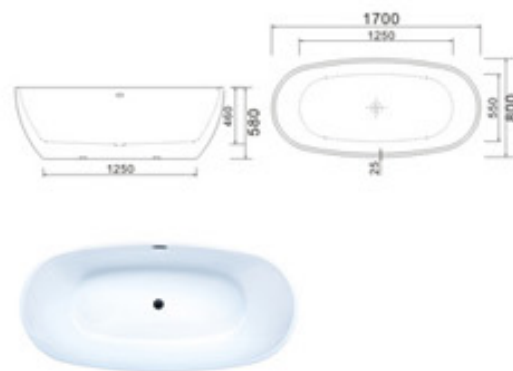
KB-531 1700x800x580mm
