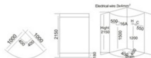
KB-854 1000x1000x2150mm
