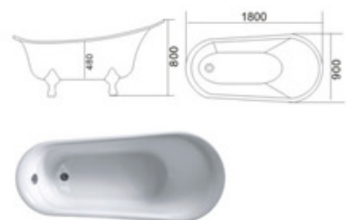
KB-553 1800x900x800mm
