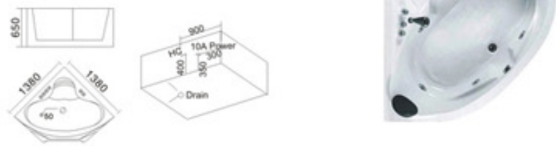
KB-652 1380x1380x650mm
