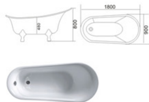
KB-552 1800x900x800mm
