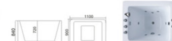
KB-2002 1100x900x840mm
