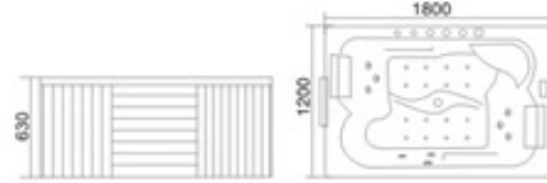
KB-634 1800x1200x630mm
