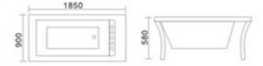
KB-527 1850x900x580mm
