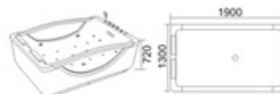
KB-602 1900x1300x720mm
