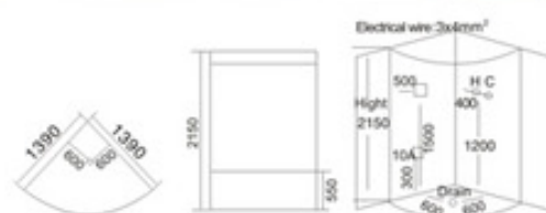
KB-709 1390x1390x2150mm
