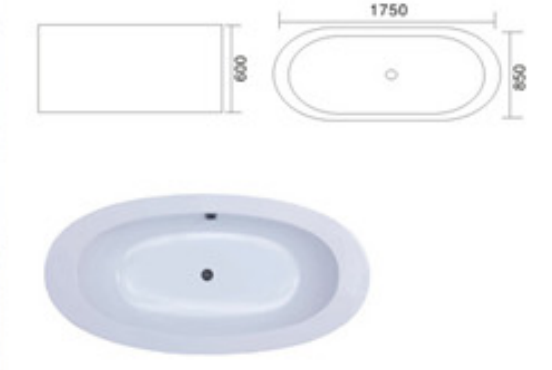
KB-523 1750x850x600mm
