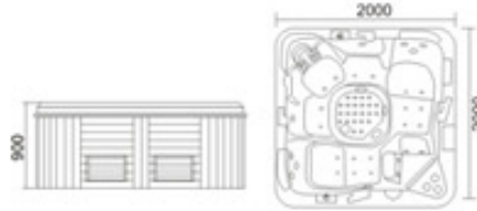
KB-207 2000x2000x900mm
