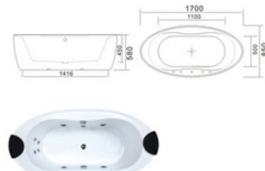
KB-520 1700x850x580mm
