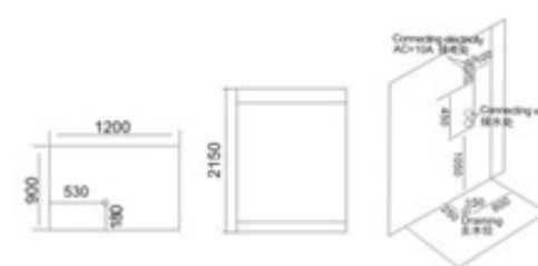
KB-857 1200x900x2150mm
