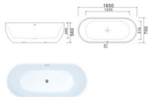
KB-530 1650x700x560mm
