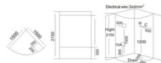
KB-856 1500x1500x2150mm
