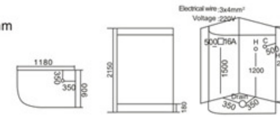
KB-704 1200x900x2150mm
