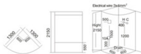
KB-855 1300x1300x2150mm
