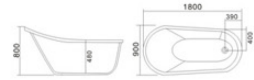
KB-518 1800x900x800mm
